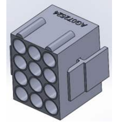
12 WAY LUCAS/RISTS SOCKET HOUSING REPL: 51150010 AG072524
